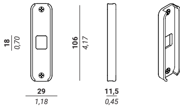
Dimensioni contropiastra / Counterplate dimensions
